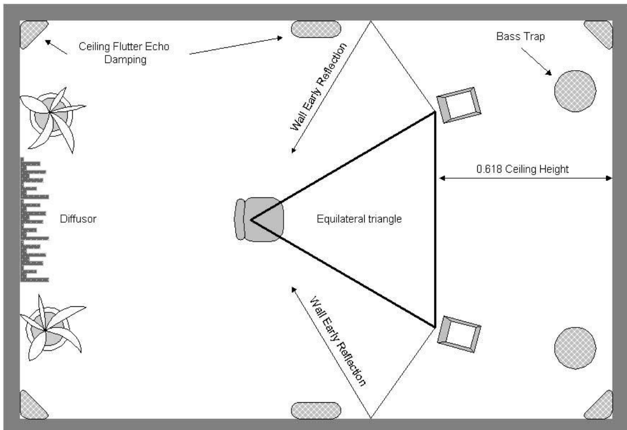
Figure 1 Room placement method number 1 and different room treatment devices
